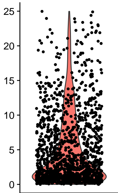
percent.mt
