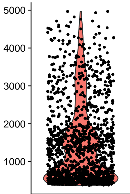
nFeature_RNA
