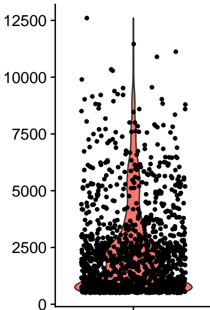
nCount_RNA
