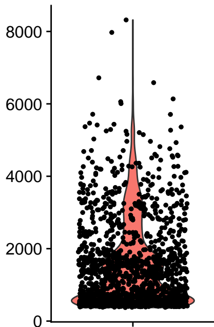
nFeature_RNA
