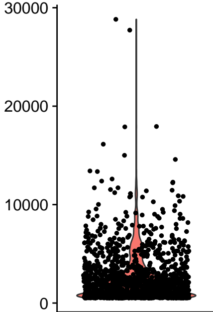
nCount_RNA
