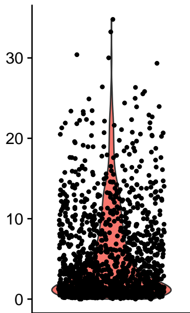
percent.mt
