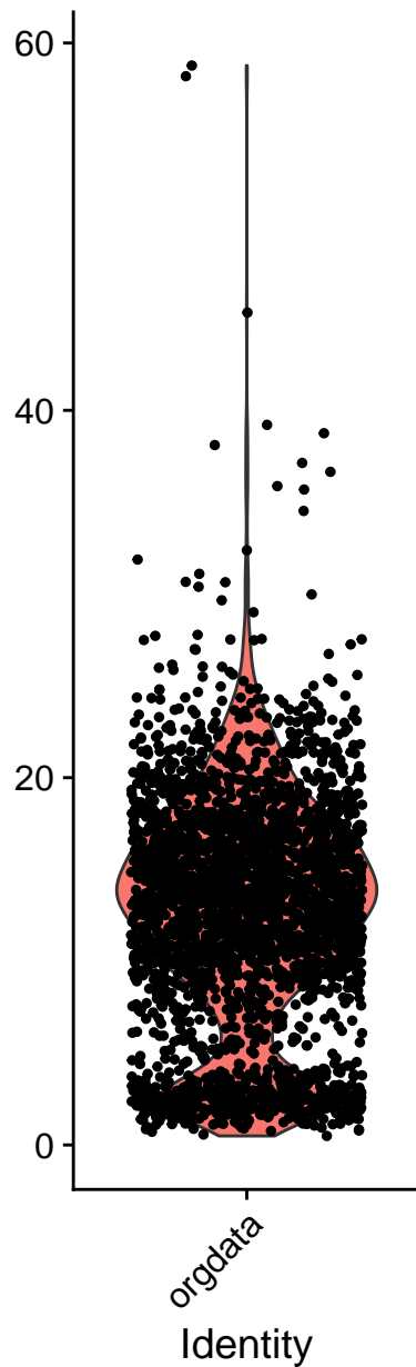
percent.mt
