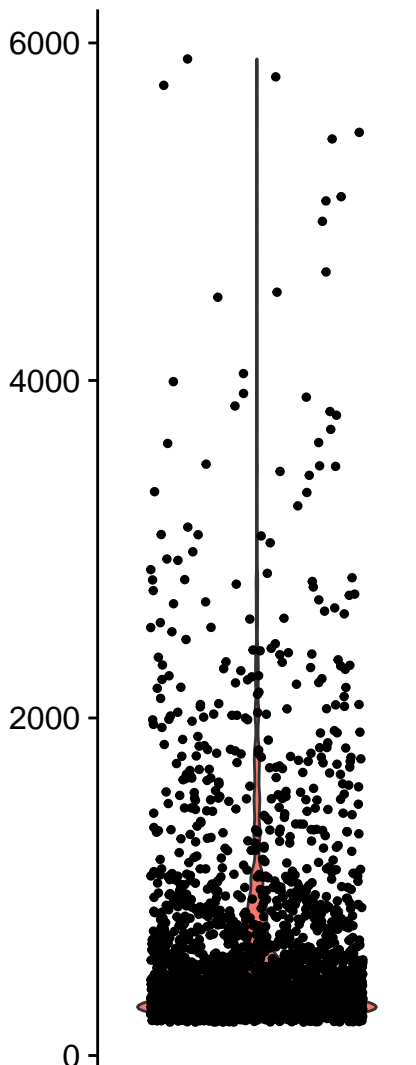
nFeature_RNA
