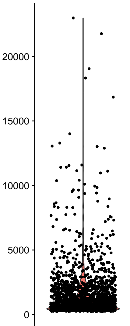
nCount_RNA
