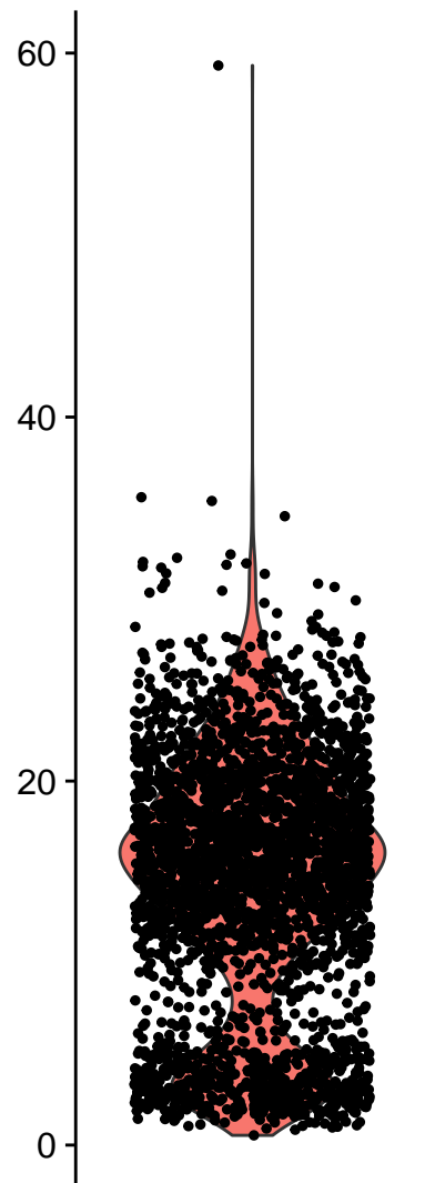
percent.mt
