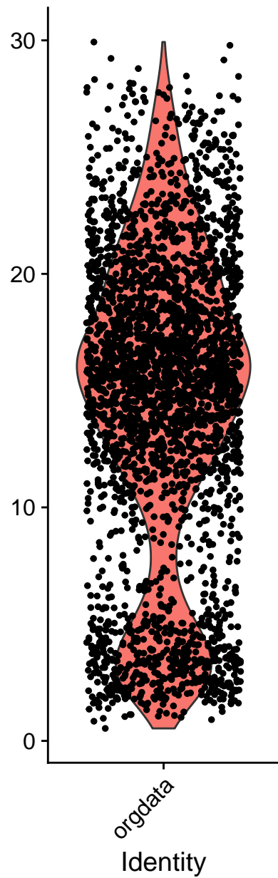
percent.mt
