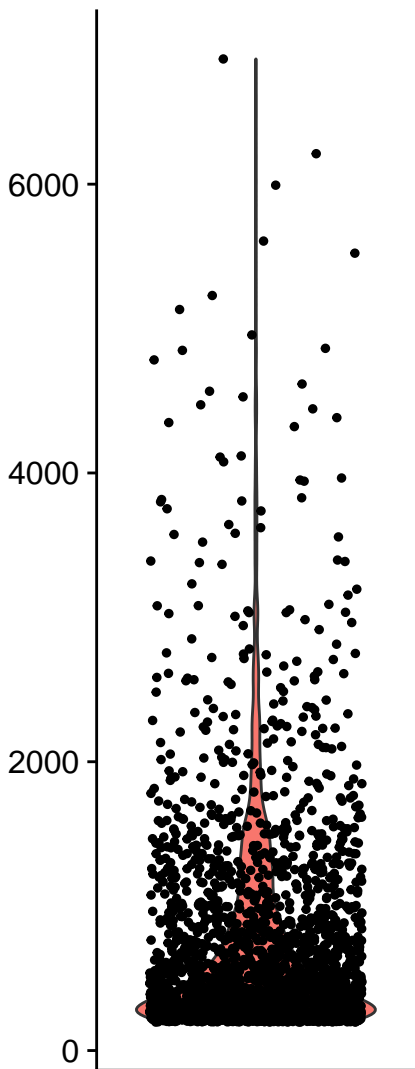
nFeature_RNA
