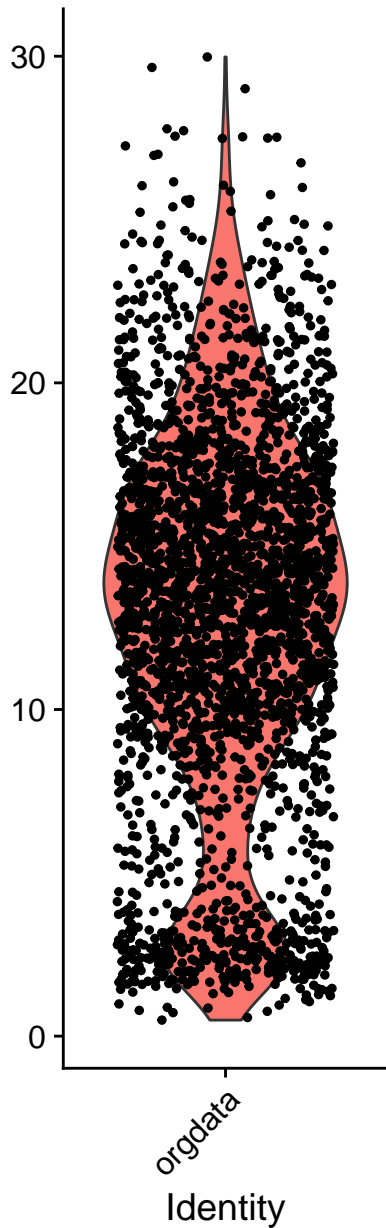
percent.mt
