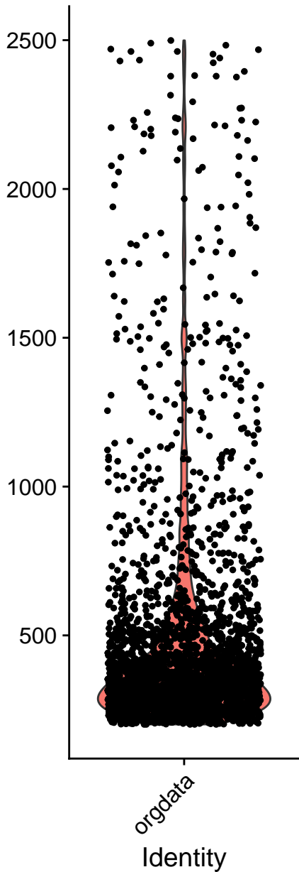
nFeature_RNA
