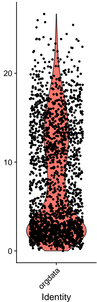
percent.mt
