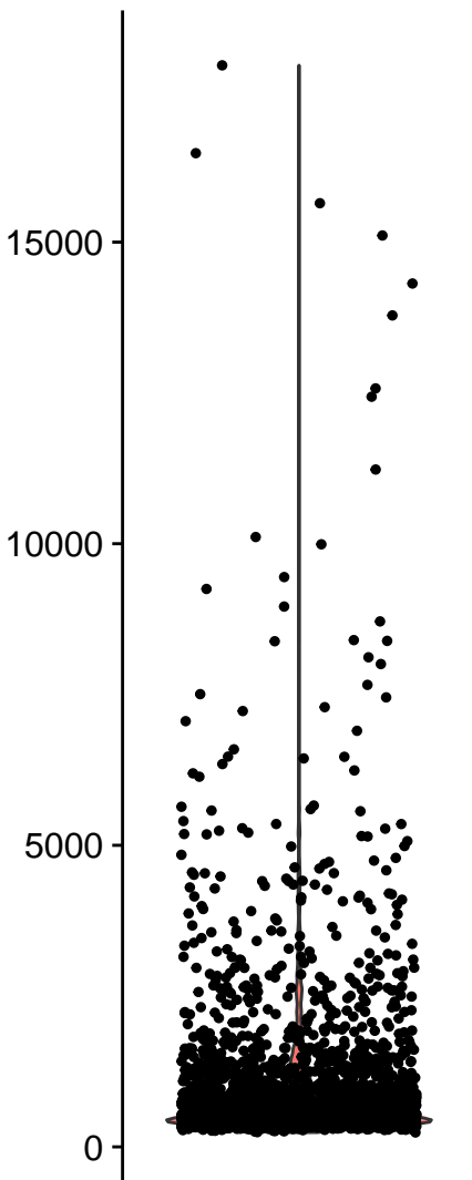
nCount_RNA
