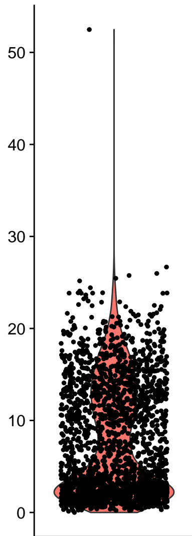
percent.mt
