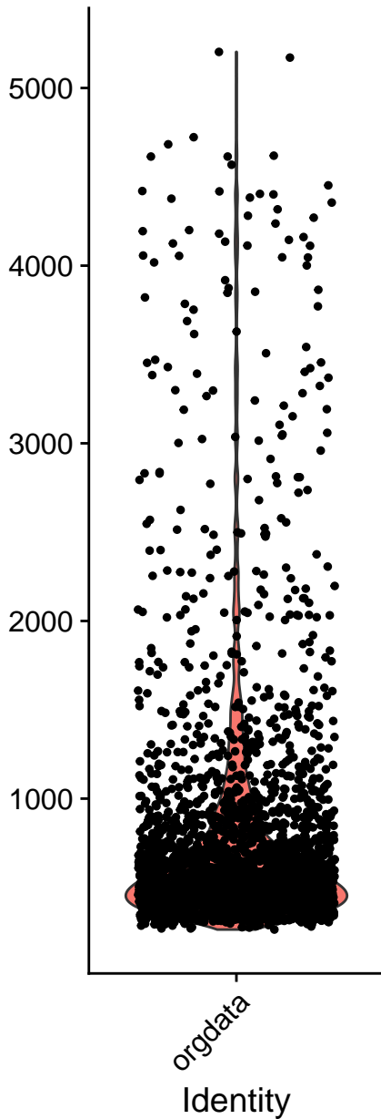
nCount_RNA
