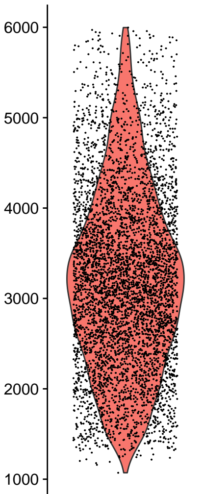
nFeature_RNA
