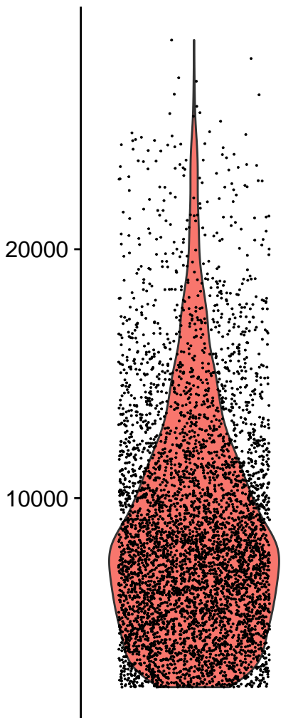
nCount_RNA
