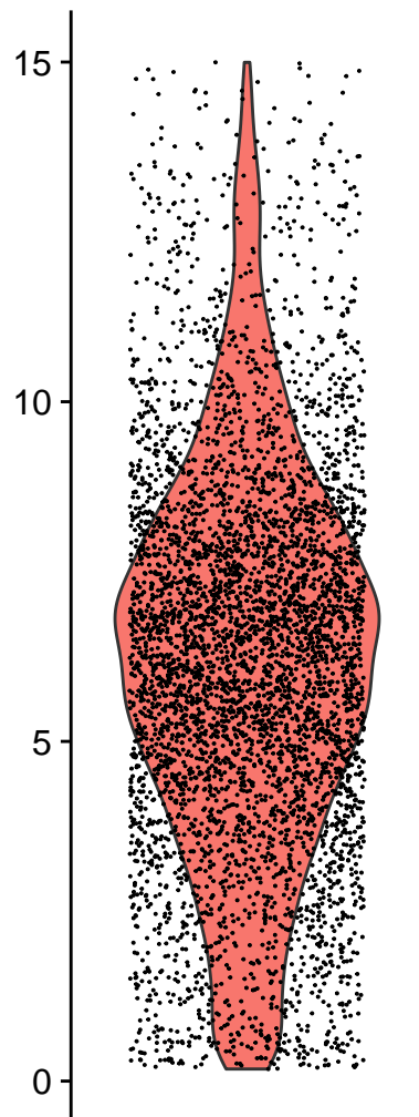
percent.mt
