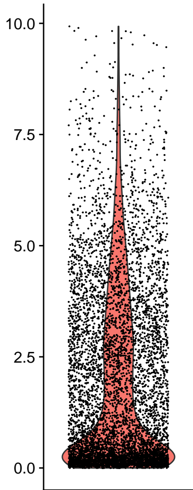
percent.mt
