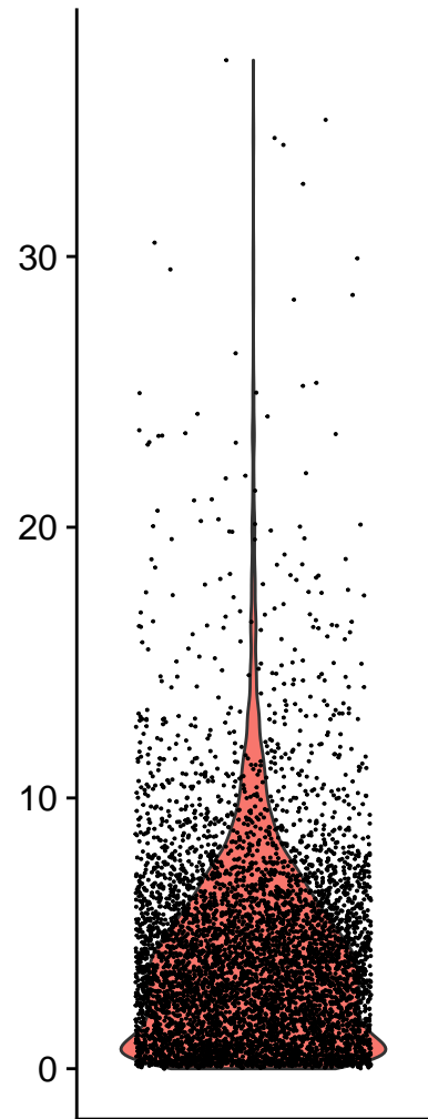
percent.mt
