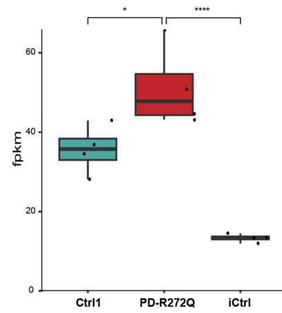
B) Dopaminergic neurons RHOT1 expression levels
