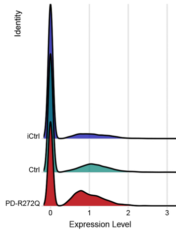
A) Midbrain organoids RHOT1 expression levels
