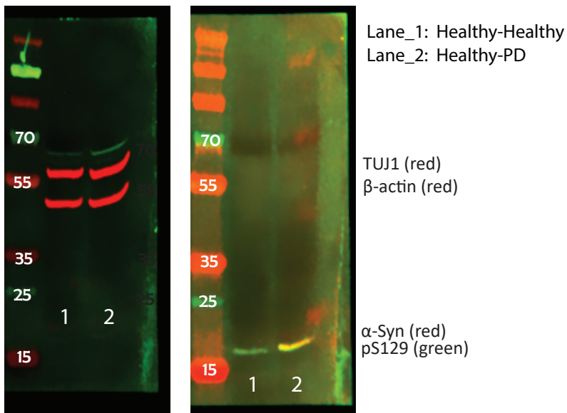
E Uncropped membrane from Figure S4G
