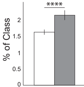
PI (36:1)
