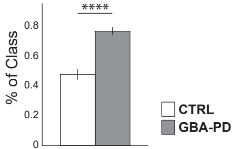
PI (40:4)
