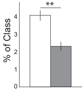
PI(38:5)
